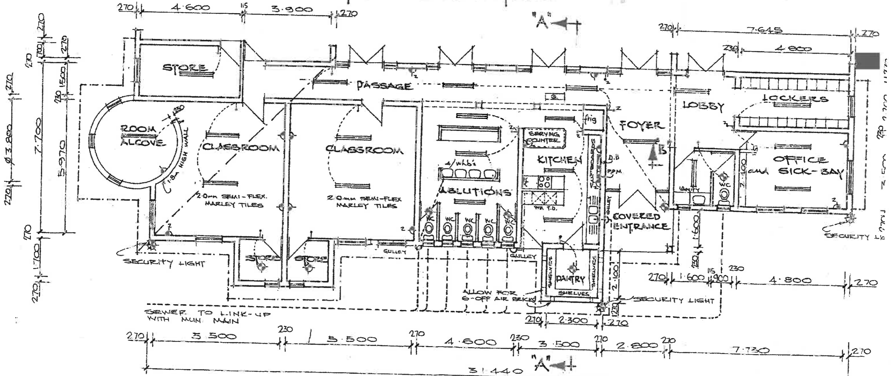
FLOOR PLAN
